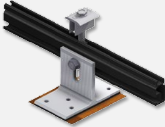
SOLARMOUNT BUTYL ATTACHMENT
