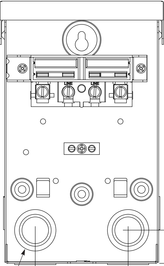
View Shown With Shield Removed
