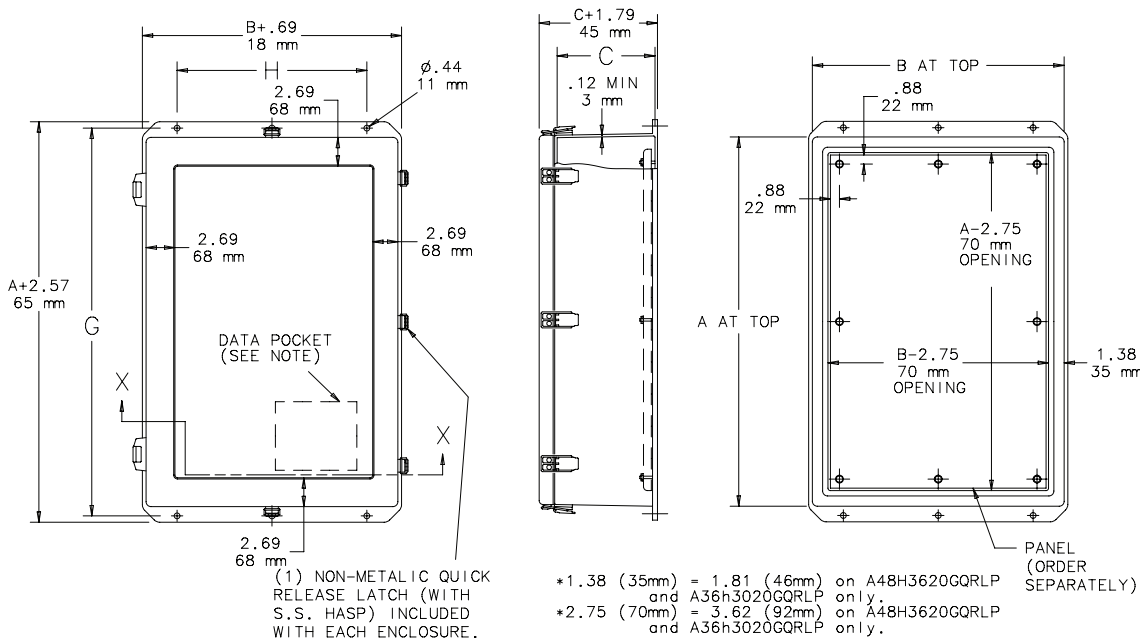
Hinged with Quick-Release Latch Enclosures 36 X 36 or Larger Drawing 4)
