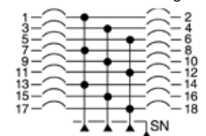
3 Phase, 4 Wire, 3 Phase 3 Wire (No SN)
