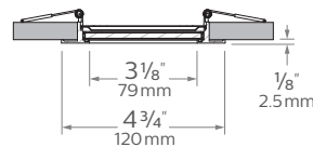
Flat Downlight 4" Round
