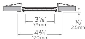
Flat Downlight 4" Square
