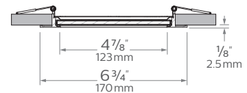
Flat Downlight 6" Round
