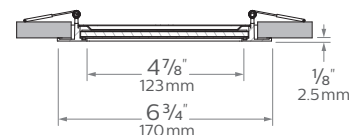
Flat Downlight 6" Square
