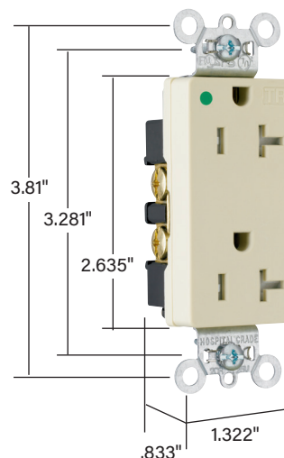
Dimensions for 15 & 20 Amp TR26362HGI
