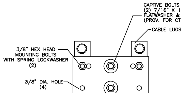
ø BUS DETAIL
