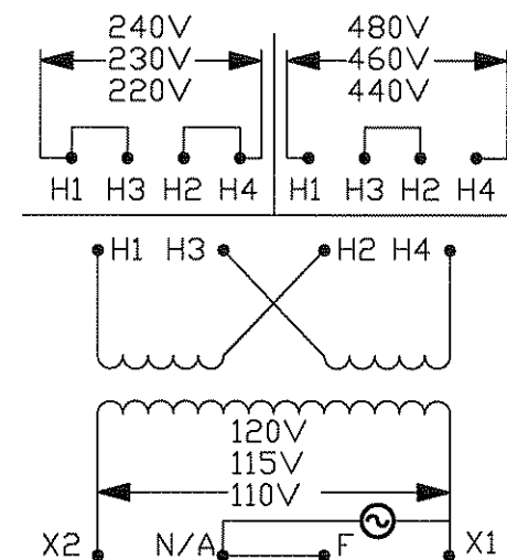
CONNECTION DIAGRAM
