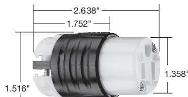
Dimensions for 15 & 20 Amp Connector
