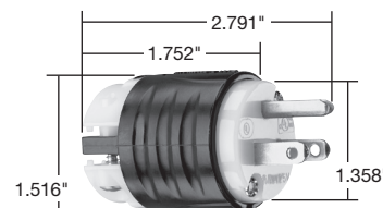
Dimensions for 15 & 20 Amp Plug
