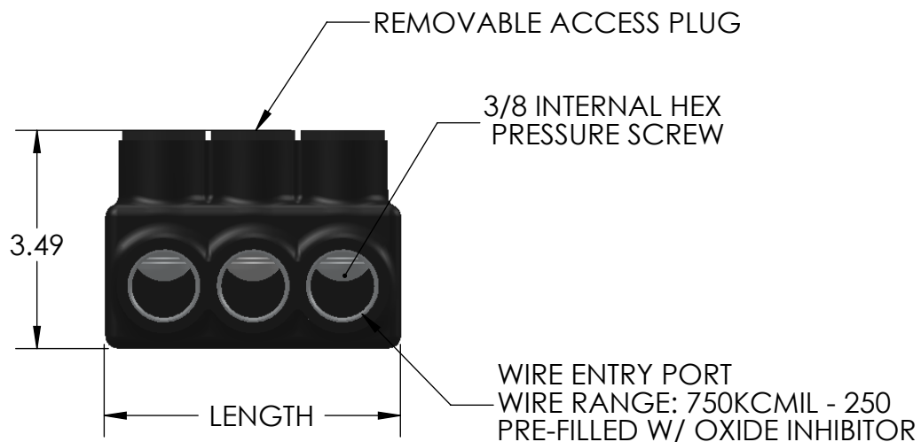
IPL750-3 SHOWN
