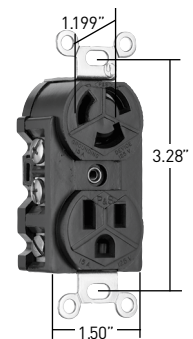
Dimensions for 4792
