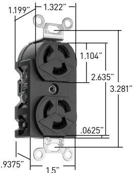
Dimensions for 4700
