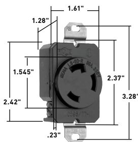
Dimensions for 30 Amp Receptacle
