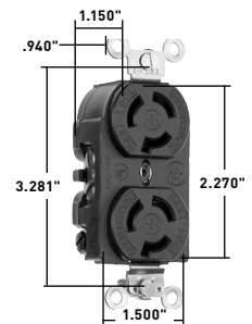
Dimensions for 4550
