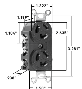
Dimensions for 4750
