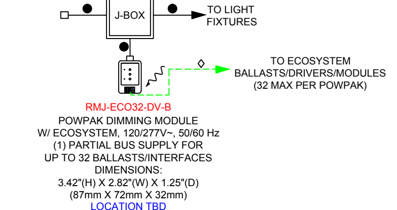
RMJ-ECO32-DV-B WITH JBOX
