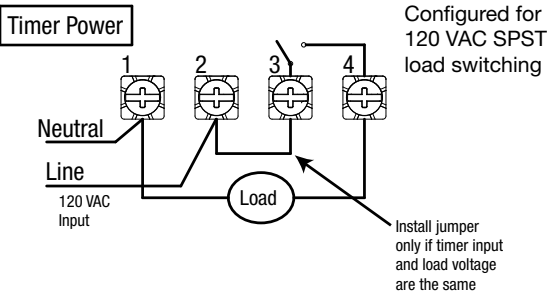
Wiring diagrams for ET1125C/CR/CPD82, ET1725C/CR/CPD82, ET8215C/CR/CPD82
