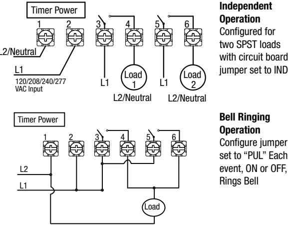
Wiring diagrams for ET1125C/CR/CPD82, ET1725C/CR/CPD82, ET8215C/CR/CPD82
