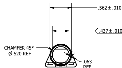
DETAIL A, SCALE 1.8 : 1 TOP INK MARKING INK COLOR: BLACK PER SPEC #: F921
