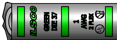
DETAIL A, SCALE 2 : 1 TOP & BOTTOM INK MARKING INK COLOR: GREEN PER SPEC #: F921
