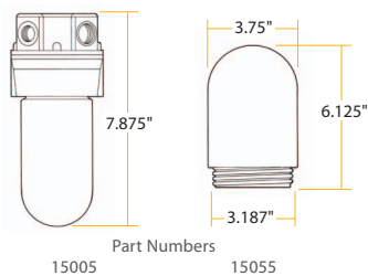
Fixture Globe and Junction Box Dimensional Reference
