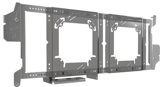
Telescoping bracket with box mounting brackets installed
