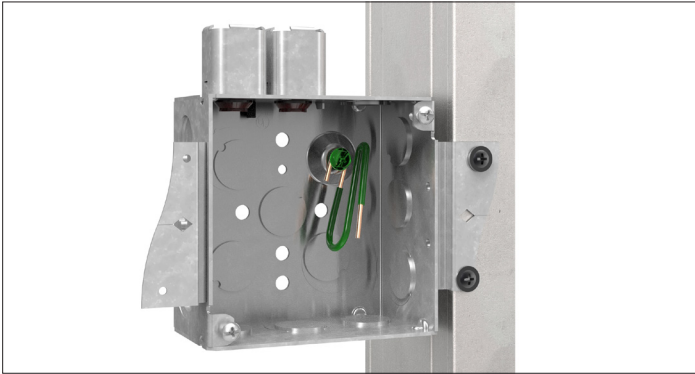
Step 1. Mount box to stud.
